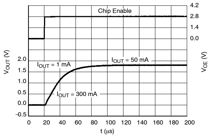
Figure 81. Start-up, 1.8 V Version, V_{IN} = 2.8 V
